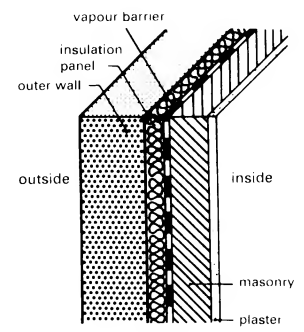
④ Wall with internal vapour barrier
